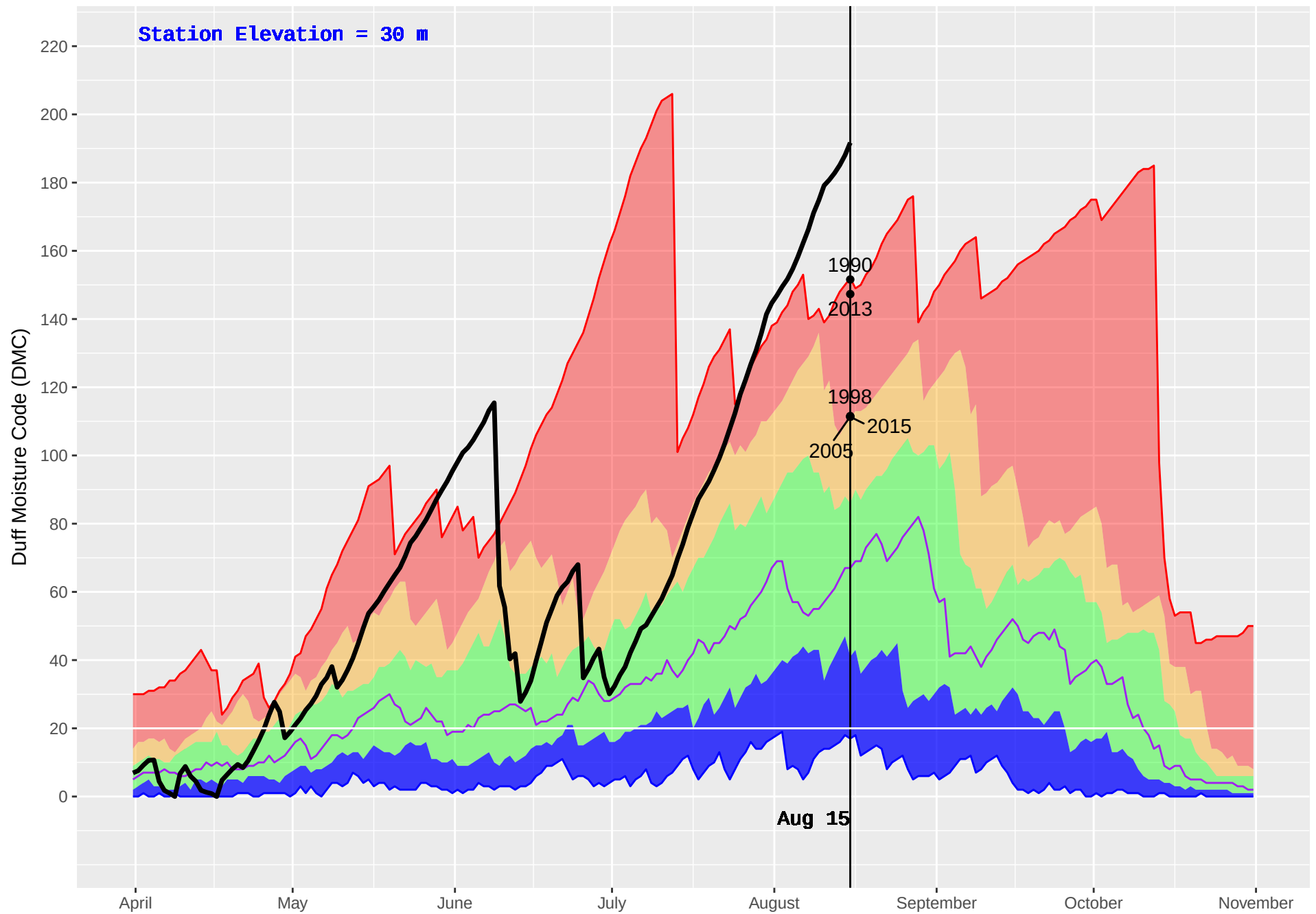
CEDAR (59) : Historical (1989–2016) and Current (2018) Daily Duff Moisture Code (DMC)
